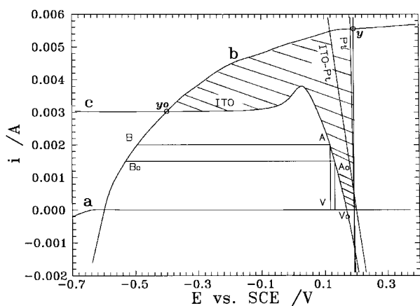
Fig. 2. I/V curve of \alpha\text{-PbO} | 0.1 \text{ M Fe}(\text{CN})_6^{4-}, 0.01 \text{ M Fe}(\text{CN})_6^{3-} | : (a) In dark, (b) under white light illumination. Curve (c) is the I/V curve of the ITO in 0.1 M \text{Fe}(\text{CN})_6^{4-} , 0.01 M \text{Fe}(\text{CN})_6^{3-} solution (Figure 1(a)).
