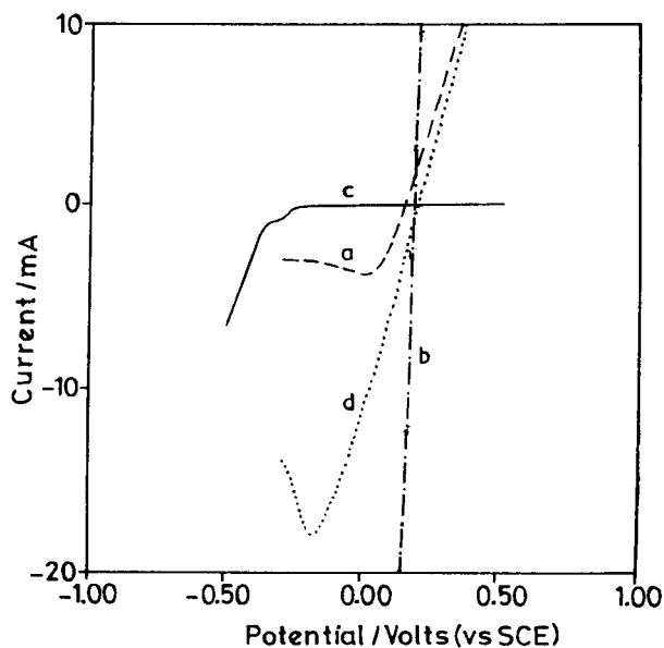
Fig. 1. (c) Cathodic half cycle plot of ITO electrode in 10^{-2} M \text{H}_2\text{PtCl}_6 solution (i.e., for surface modification of ITO electrode with platinum). I/V curve in 0.1 M \text{Fe}(\text{CN})_6^{4-} , 0.01 M \text{Fe}(\text{CN})_6^{3-} solution with (a) ITO electrode, (b) Pt electrode, (d) surface modified ITO electrode with platinum.
